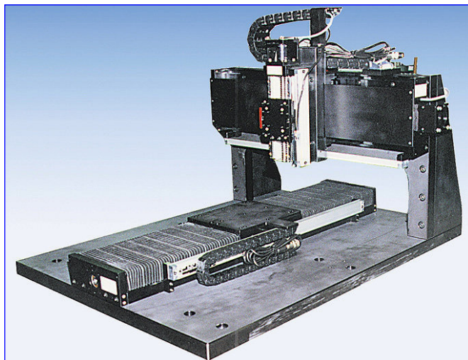
X-Z vision inspection station mounted on steel sub plate
