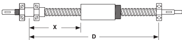
Rigid-Simple
