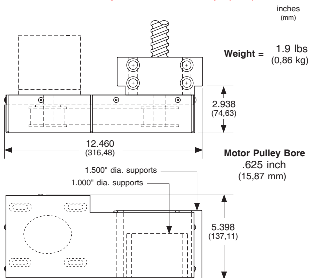
NEMA 42 Right Hand Motor Wrap (M12)
