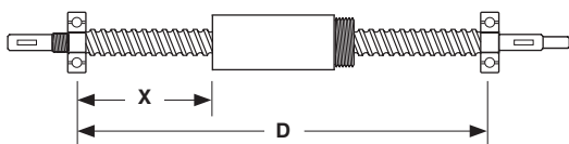
Simple-Simple
